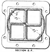
Figs. 373-375. Exhaust Pipe for Ten-Wheel (4-6-0) Locomotive with Cleveland Cylinders. Intercolonial Railway.
